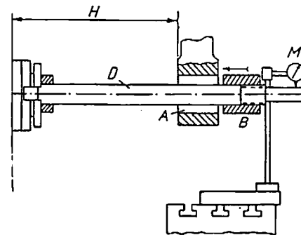
Fig. 53. Slip-bushing Method
