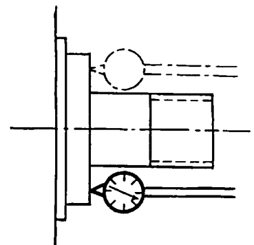
Fig. 44. Testing the Face of a Shoulder
