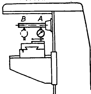
Fig. 63. Parallelism between the Surface of the Table and the Spindle Axis
