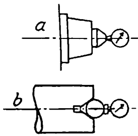
Fig. 45. Axial Slip of a Spindle
