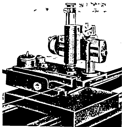
Fig. 8. Method of Testing by means of a Taut Wire and Measuring Microscope
