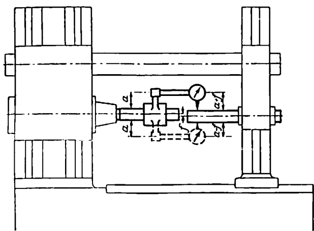
Fig. 19. (See page 31 and Fig. 1A-C). Tolerances in Testing the alignment of Two Axes by the Swing-over Method
