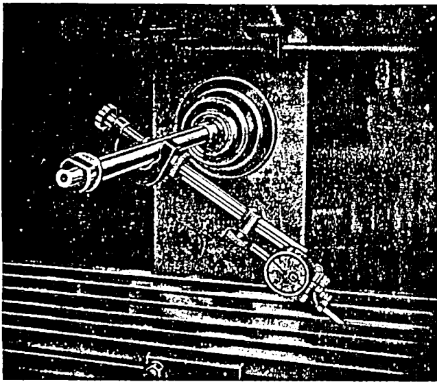
Fig. 66a. Set-up for Checking T-slots
