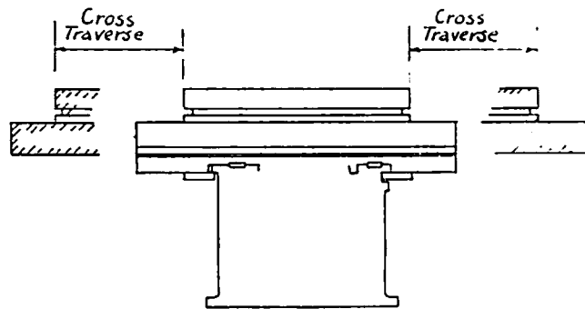
Fig. 29. Table with Length equal to that of the Slideway
