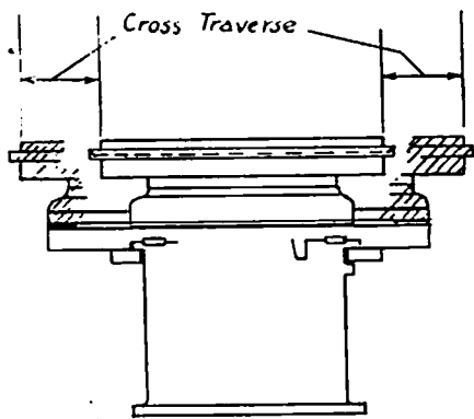
Fig. 28. Table that is Shorter than its Slideway by an amount equal to the Cross-traverse of the Table
