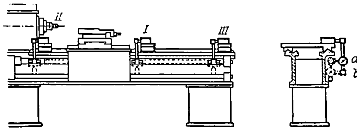
Fig. 58. Lead-screw
