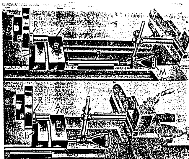
Fig. 20A (Top); Fig. 20B (Bottom). Method of Measuring Lead-screw Errors by Comparison with an End Gauge.
