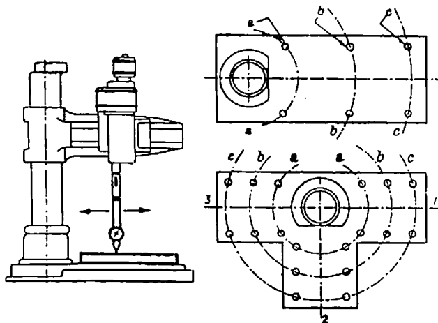
Fig. 85A. Parallelism of Drilling-head Slideways and Base
