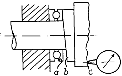
Fig. 43. Testing Axial Slip
