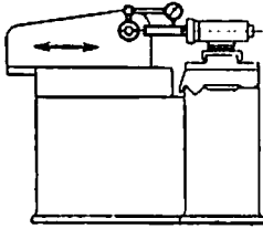
Fig. 73. Parallelism between the Spindle Axis and the Direction of the Infeed Movement (Universal Grinding Machines)
