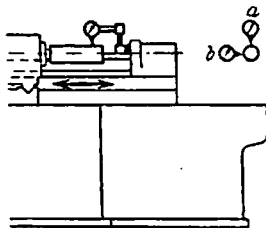
Fig. 75. Testing Parallelism between Grinding-wheel Spindle and Table Movement
