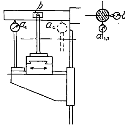
Fig. 68. Checking the Parallelism of Overarm with Transverse Movement
