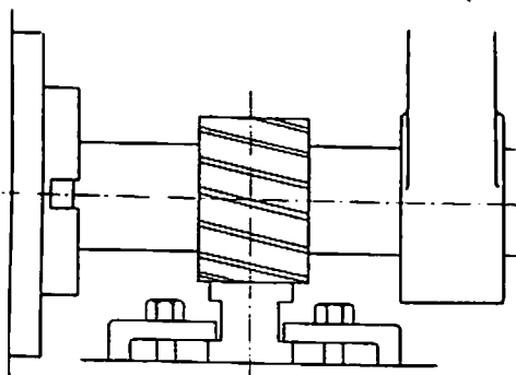
Fig. 90a. Performance Test on Milling Machine—Slab Milling
