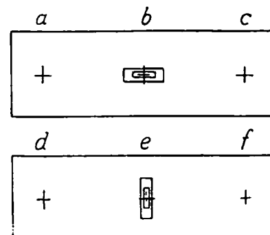
Fig. 31. Levelling the Table of a Milling Machine
