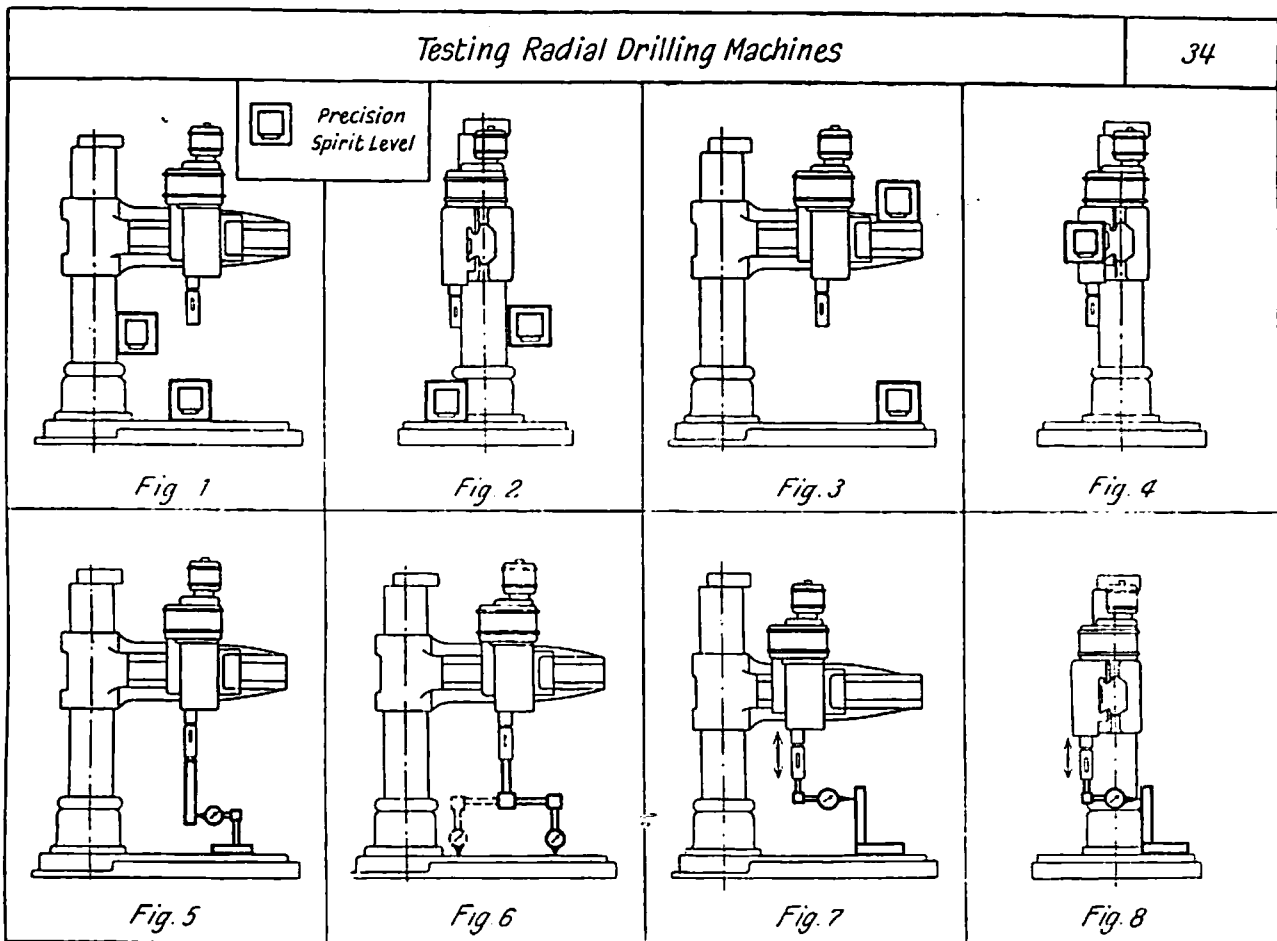
Test Chart for Multi-spindle Drilling Machines with Universal-joint Driven Spindles | No. 33 Chart 2
