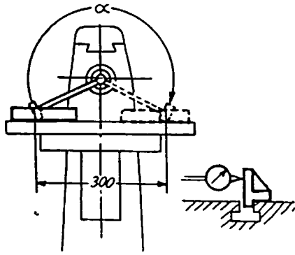
Fig. 70. Perpendicularity between the Centre T-slot and the Spindle
