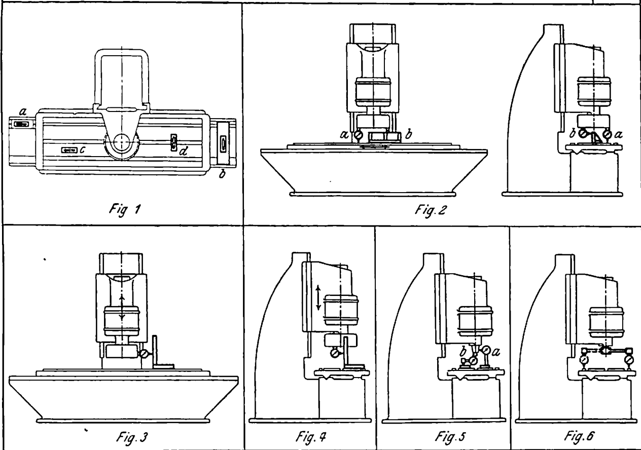
Test Chart for Vertical Surface Grinders
