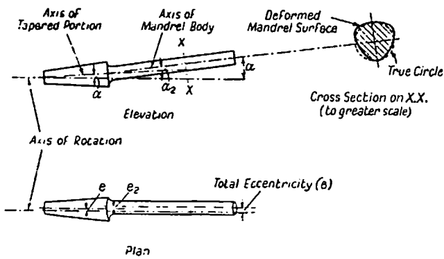
Fig. 41. Sources of Error in Rotating Mandrels
