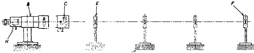
Fig. 11. General Arrangement of Optical Alignment Testing Telescope
