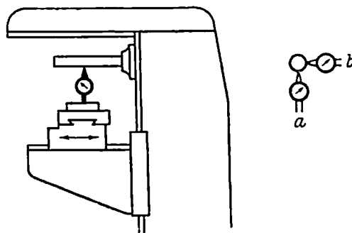
Fig. 65. Transverse Movement of Table parallel with Spindle Axis
