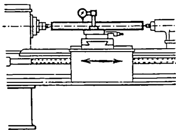
Fig. 60. Height of Centres
