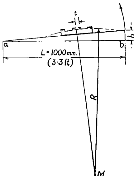
Fig. 5A. Sensitivity of Spirit Level
