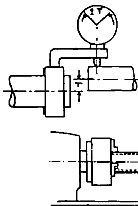
Fig. 48. Tubular Holder for Dial Gauge
