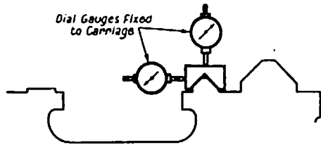
Fig. 26. Checking the Parallelism of Guideways
