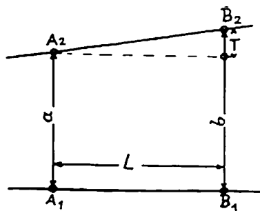
Fig. 54. Checking for Parallelism
