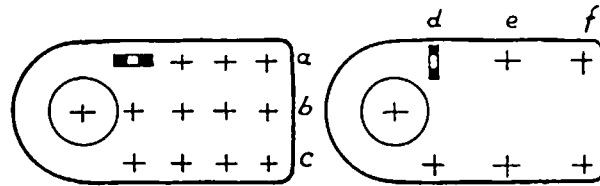
Fig. 39A and 39B. Checking Flatness of Base
