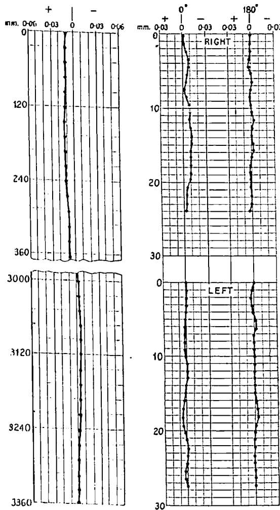
Fig. 22 (Left). Test Chart for an Accurate Lead-screw
