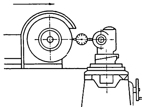
Fig. 90c. Fine In-feed Test
