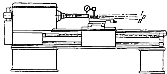
Fig. 4. Mandrel running out of Truth must be set to Mean Position before Testing for Parallelism with the Bed
