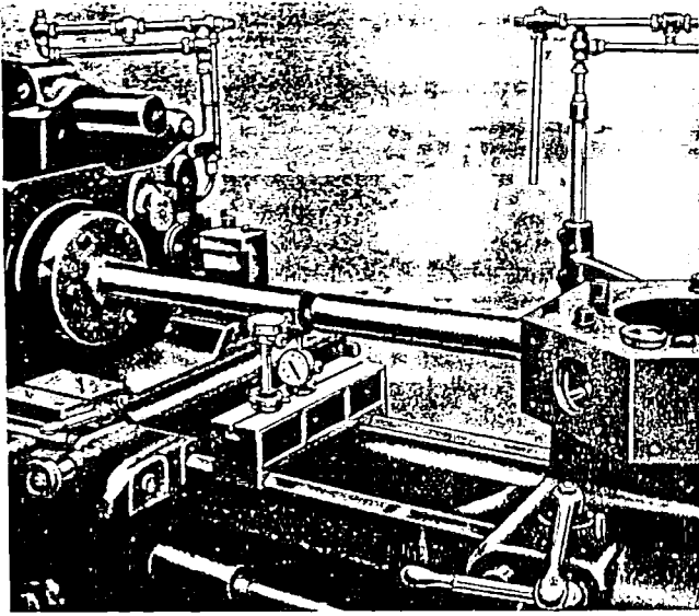
Fig. 50. Arrangement of Double Mandrel Test
