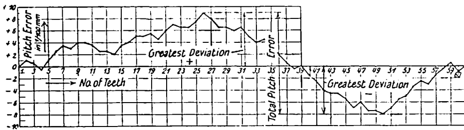
Fig. 25. Diagram of Pitch Errors of a Dividing Gear
