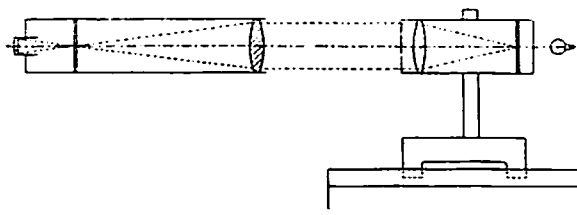
Fig. 10. Diagram illustrating the Principle of Testing by means of Target and Telescope
