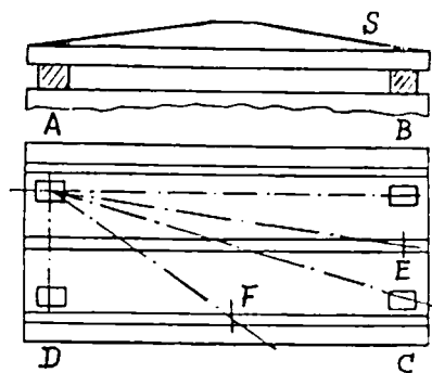
Fig. 36. Checking Flatness of Table
