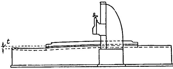
Fig. 14. Tolerances in Measuring the Difference of Height or Sag of a Planer Bed
