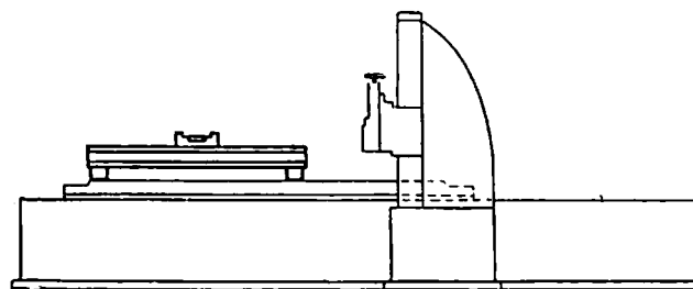
Fig. 6B. Testing Inclination of Bed with Parallels, Straight-edge and Spirit-level
