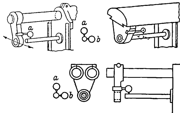
Fig. 69. Parallelism between Overarm and Spindle Axis
