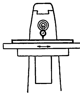
Fig. 64. Parallelism between the Table Surface and the Direction of the Longitudinal Table Movement
