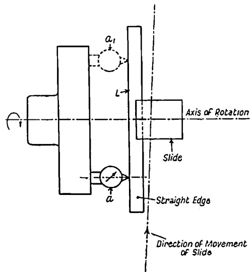
Fig. 62. Checking Perpendicularity
