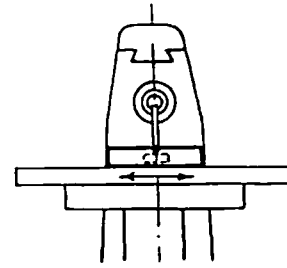
Fig. 67. Checking Parallelism of T-slot with the Table]Movement
