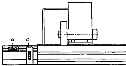
Fig. 32. Levelling the Bed of a Grinding Machine
