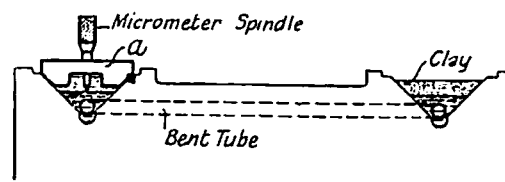
Fig. 6A. Using Vees of Bed as Water Channels when erecting Planing Machine
