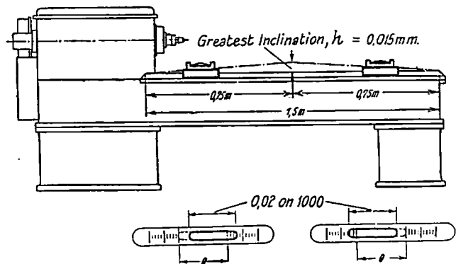
Fig. 13. Unilateral Tolerances in Spirit-level Measurements
