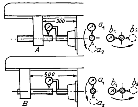
Fig. 52. Checking Spindle Alignment
