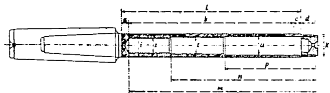
Fig. 2A. Hollow Test Mandrel with Taper Shank
