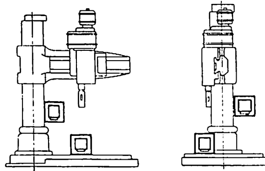
Fig. 33B and 33C. Checking the Column
