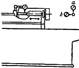
Fig. 74. Parallelism between Tailstock Sleeve and Direction of Table Traverse
