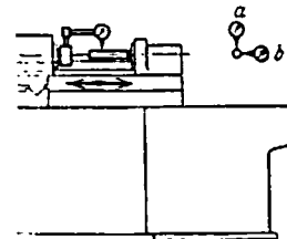
Fig. 72. Parallelism between the Spindle Axis and the Direction of the Table Traverse
