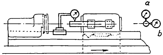
Fig. 76. Parallelism between the Internal Grinding Spindle and the Table Movement
