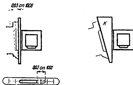
Fig. 15A. Tolerances in Testing a Surface for Flatness
