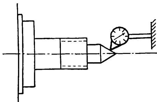
Fig. 40A. Checking the Centre
