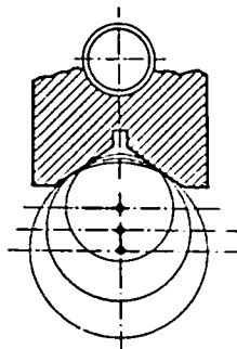
Fig. 5B. Spirit Level and Checking Cylinders
