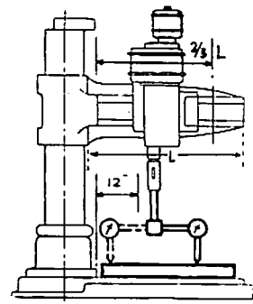
Fig. 86. Perpendicularity of Spindle
